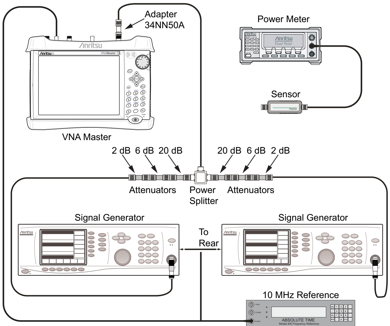
Figure 3-9. Third Order Intercept (TOI) Measurement Setup
