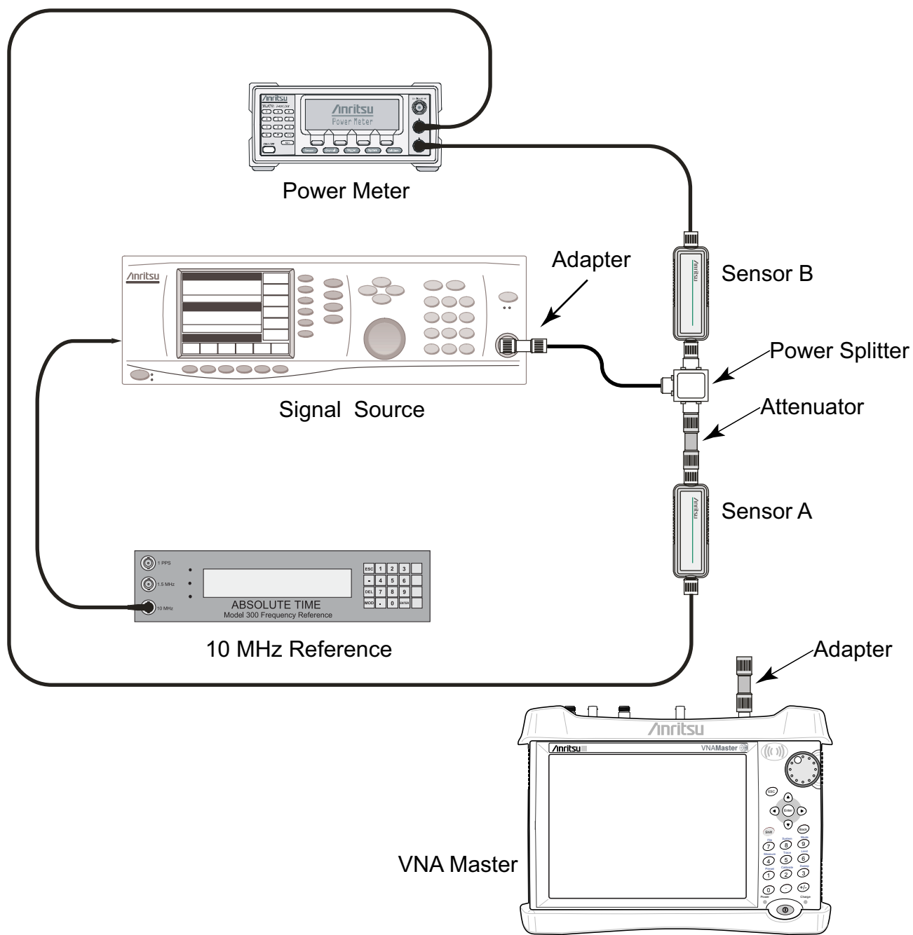
Figure 3-4. Absolute Amplitude Accuracy Verification Pretest Setup
