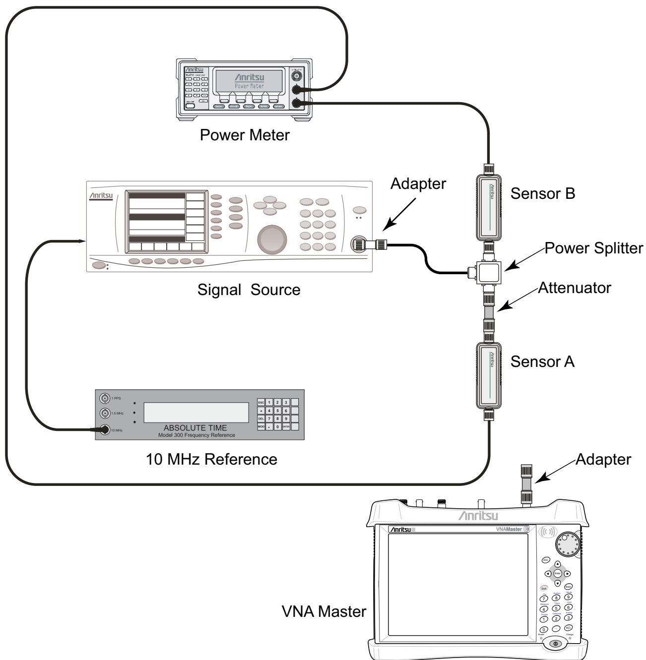
Figure 3-6. Fixed Amplitude Level with Varying Frequency Setup
