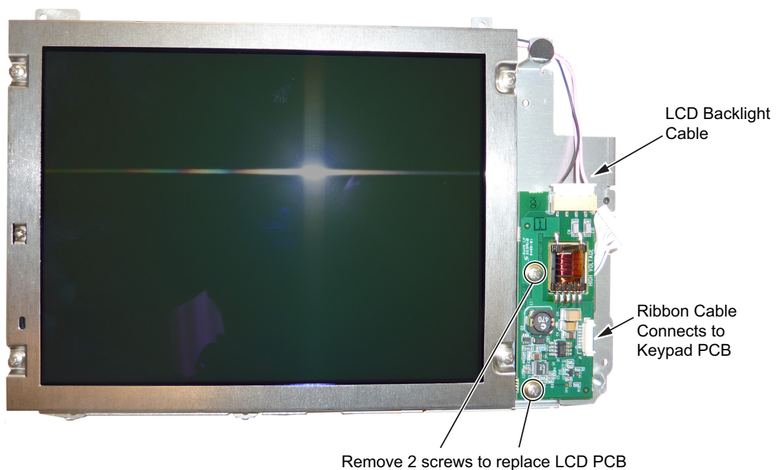
Figure 6-26. Replacing the LCD PCB
